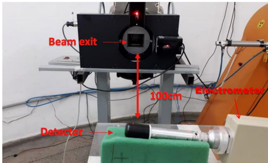
Figure 2: Measuring arrangement used in Cesa-Gammatron irradiator LCI-IPEN.
