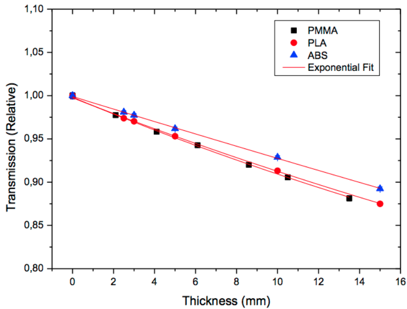
Figure 4. Comparison between the experimental transmission values of PLA, ABS and PMMA plates for different thicknesses.
