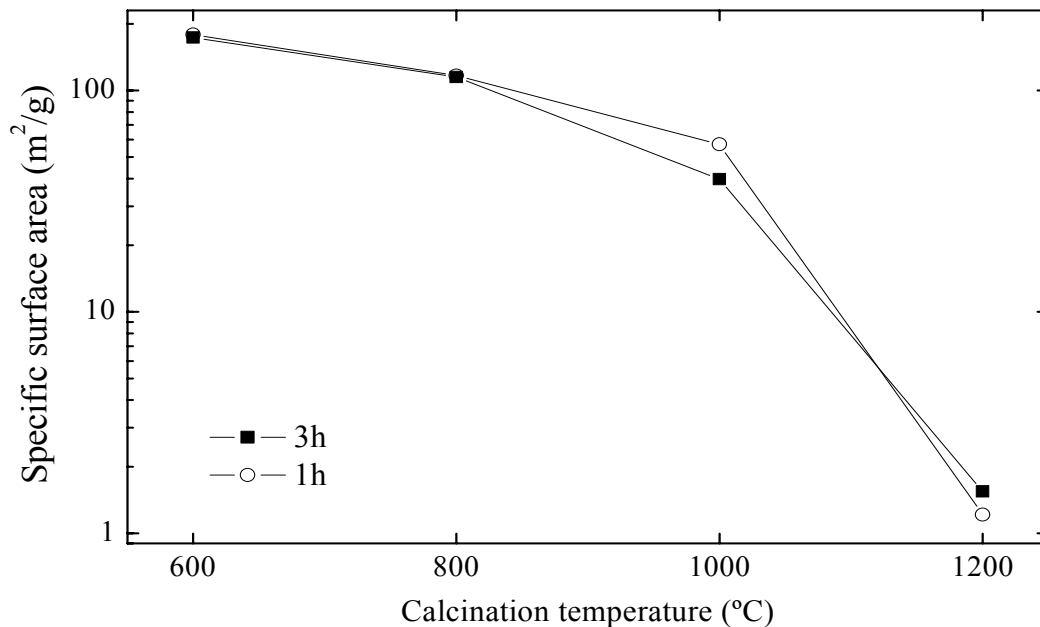
Fig.3: Specific surface area of 20 wt % \text{Al}_2\text{O}_3/\text{Y-TZP} powders, calcined in several conditions.
