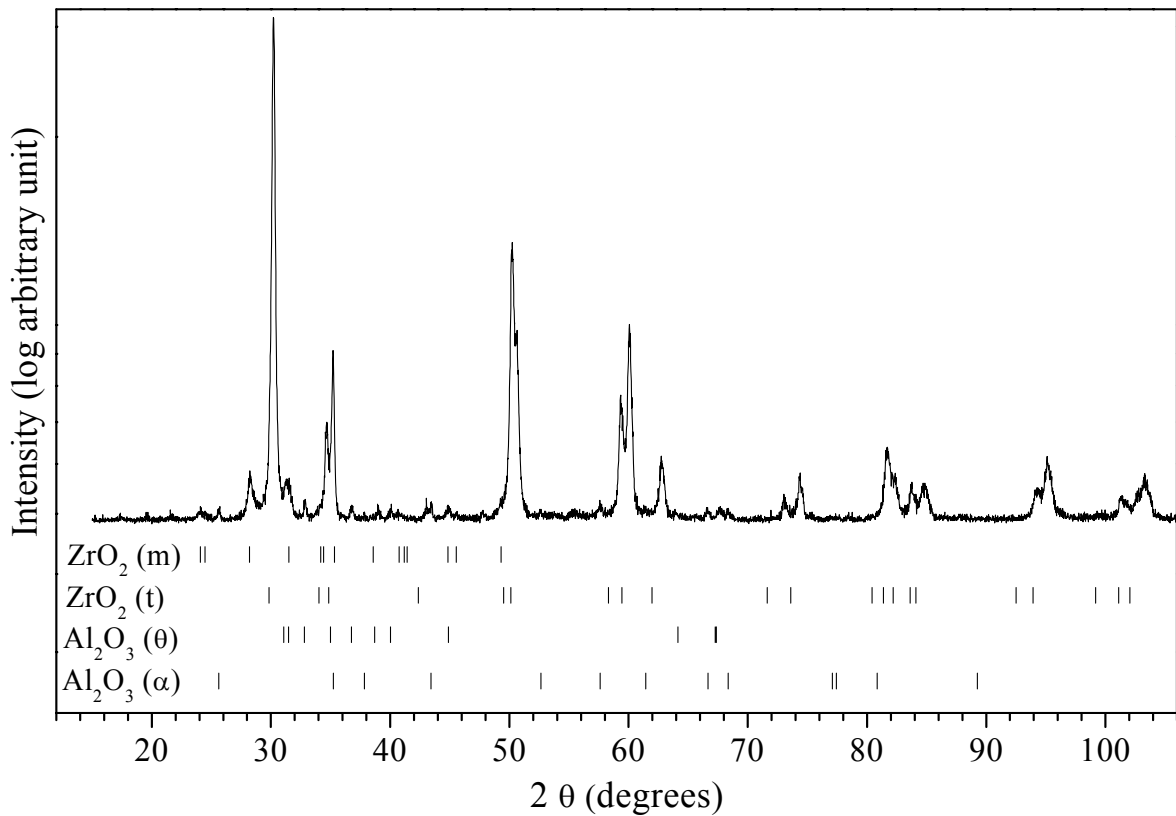
Fig.5: Diffraction pattern of 20 wt % \text{Al}_2\text{O}_3/\text{Y-TZP} powders, calcined at 1200°C for 3 hours
